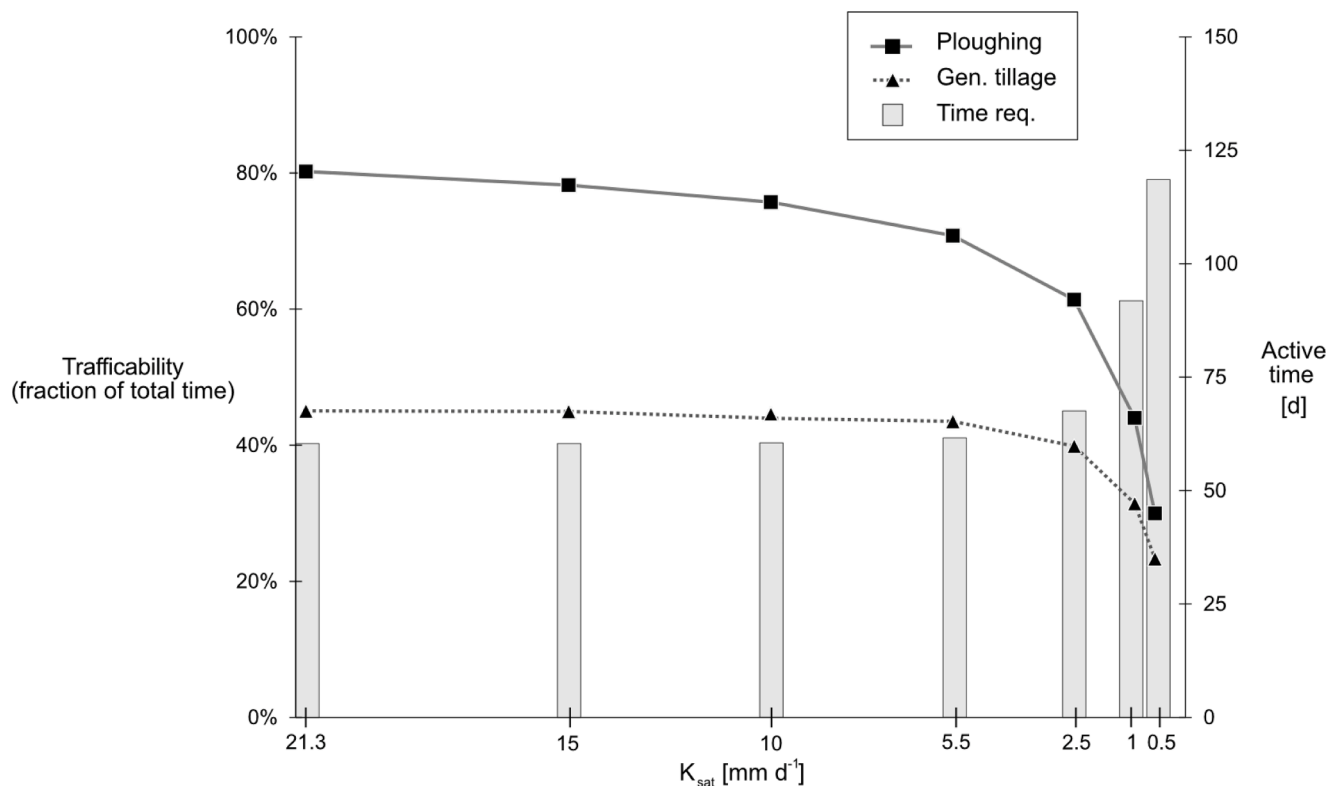
Fig. 9. Simulated trafficability and active time required for a manned 250-kW diesel tractor at different soil saturated hydraulic conductivity ( K_{sat} ) values. Trafficability (left axis) for ploughing (■) and general tillage (▲) is shown as a fraction of total time during the growing season (machine-independent). Active time required (grey bars, right axis) is also shown for an autonomous 250-kW diesel tractor.
